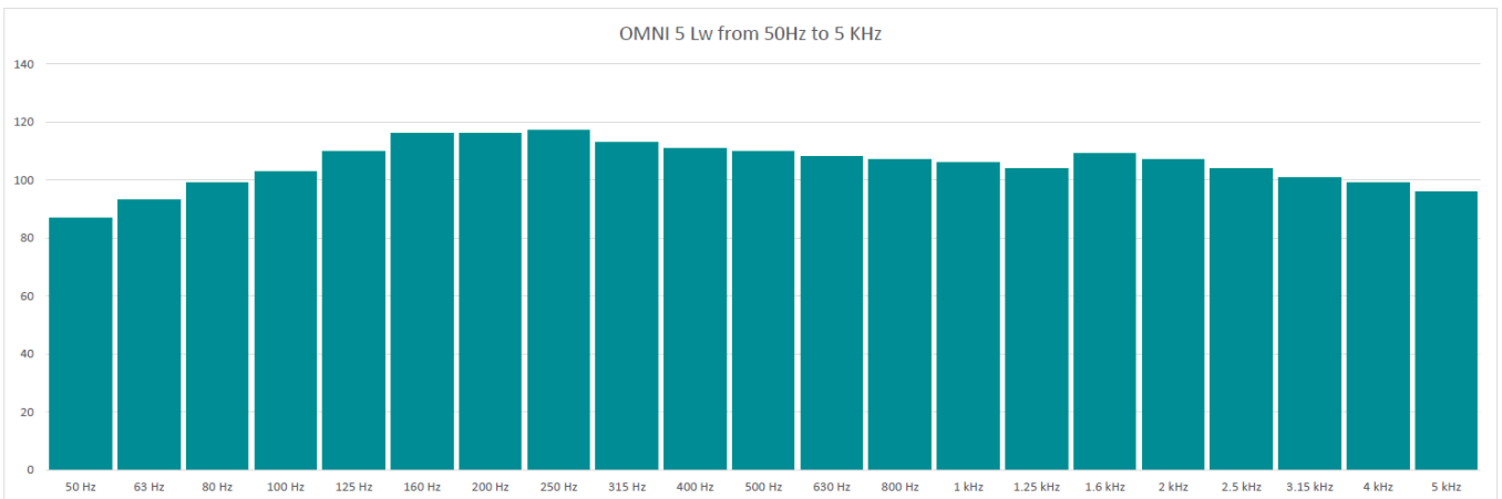
Sound Power Level (Lw) vs frequency of the Omni 5”
